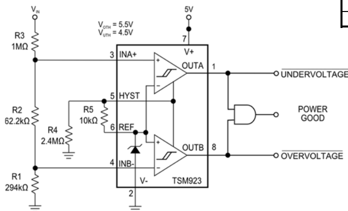
A 5V, Low-Parts-Count Window Detector
